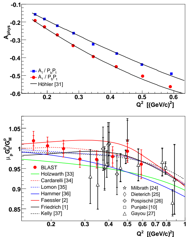
FIG. 1: Upper panel: Spin-dependent ^1\bar{H}(\vec{e}, e'p) asymmetry ( P_b P_t = 0.537 \pm 0.003 ) compared to the expected asymmetries based on the parameterization [31] for the nucleon form factors. Lower panel: Results of \mu_p G_E^p/G_M^p shown with the world polarized data [10, 24, 25, 26, 27] and several models [1, 2, 33, 34, 35, 36, 37] described in the text.
