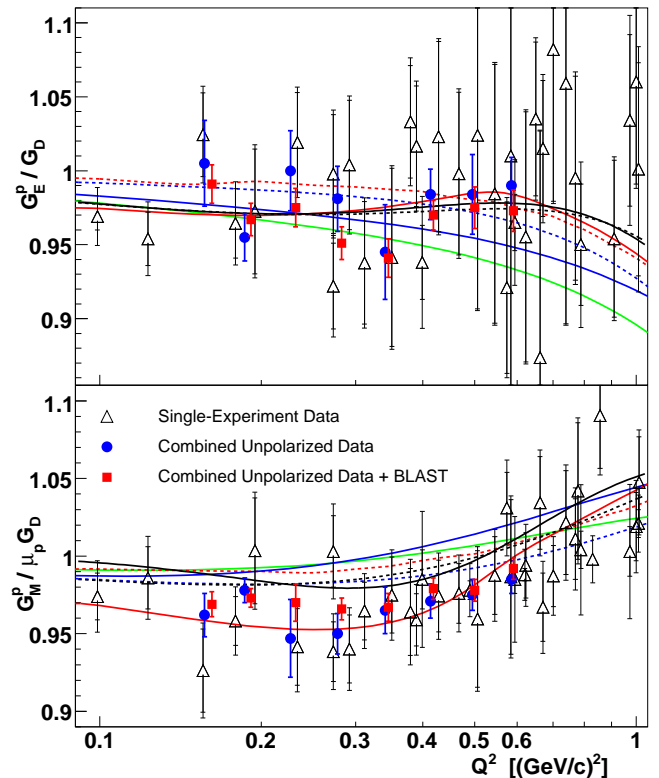
FIG. 2: Compilation of world data on G_E^p/G_D and G_M^p/\mu_p G_D at BLAST kinematics with (red) and without (blue) BLAST input, shown with total uncertainties. The results from single-experiment L-T separations [12, 14, 38, 39, 40, 41, 42, 43] are shown with open symbols. The curves have the same meaning as in Fig. 1.
